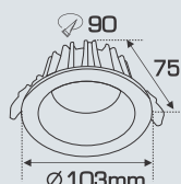
AFC 569 LED 9W 413.000
